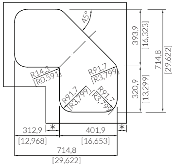
AXA D78 A
